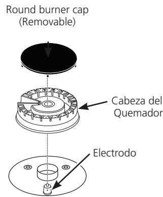
Round burner
